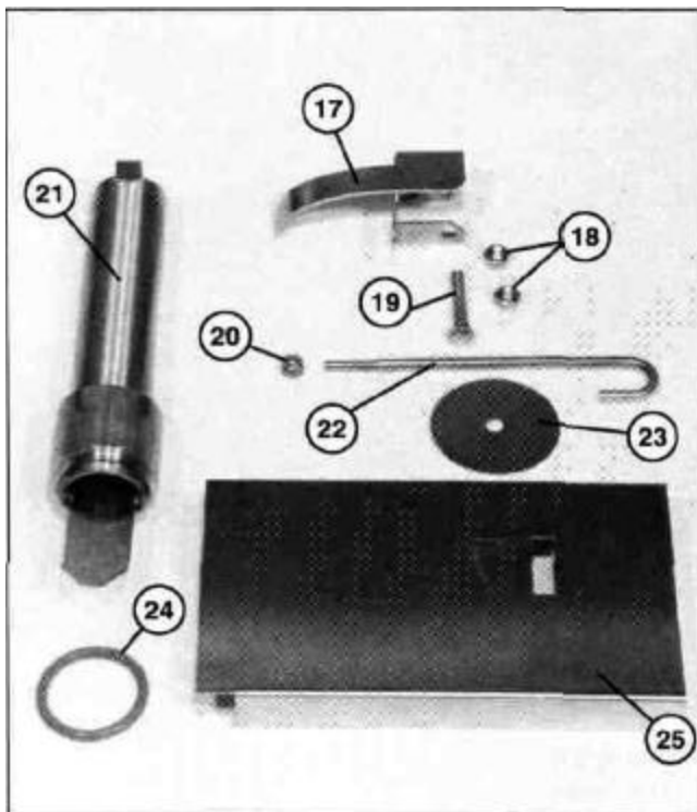
Fig. 23 - D-HB/D-H1/D-LF Track Assembly, Float Switch, and Drain Assembly
