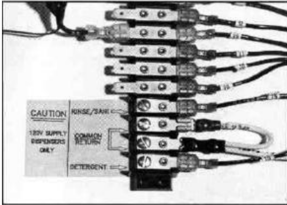
Figure 4 D-HB, D-H1, D-LF Chemical Connection Points Left Side Interior of Control Cabinet
