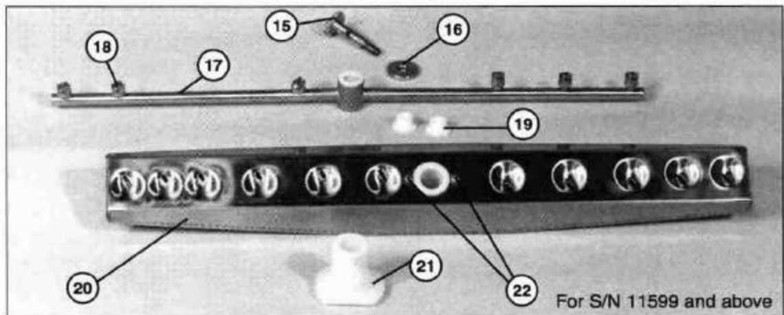
Fig. 24 - D-HB/D-H1/D-LF Wash/Rinse Spray System Assembly
