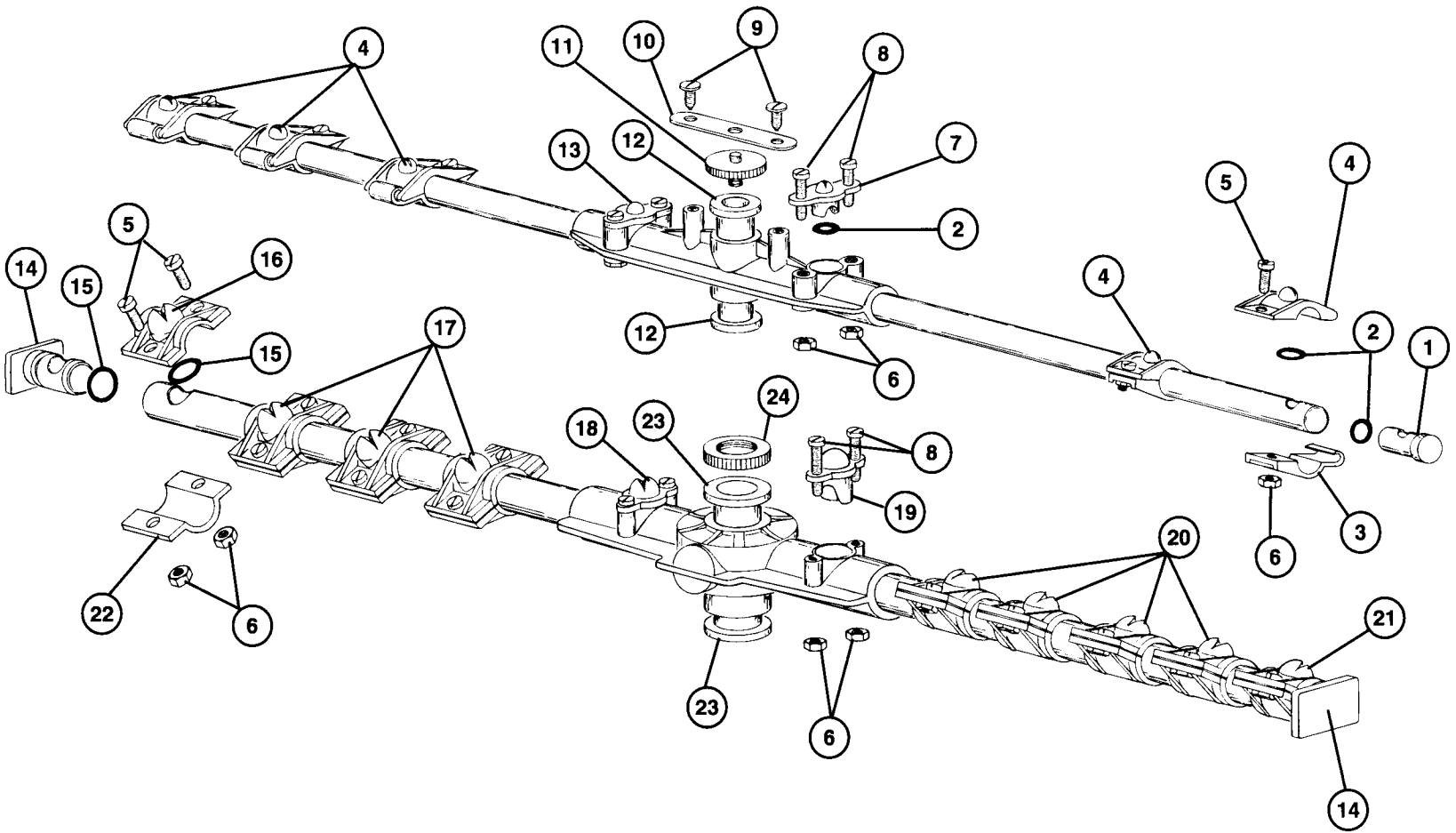
Fig. 25 - D-HB/D-HI/D-LF Wash/Rinse Spray Arms (For machines beginning with S/N 77855 through S/N 11599)
