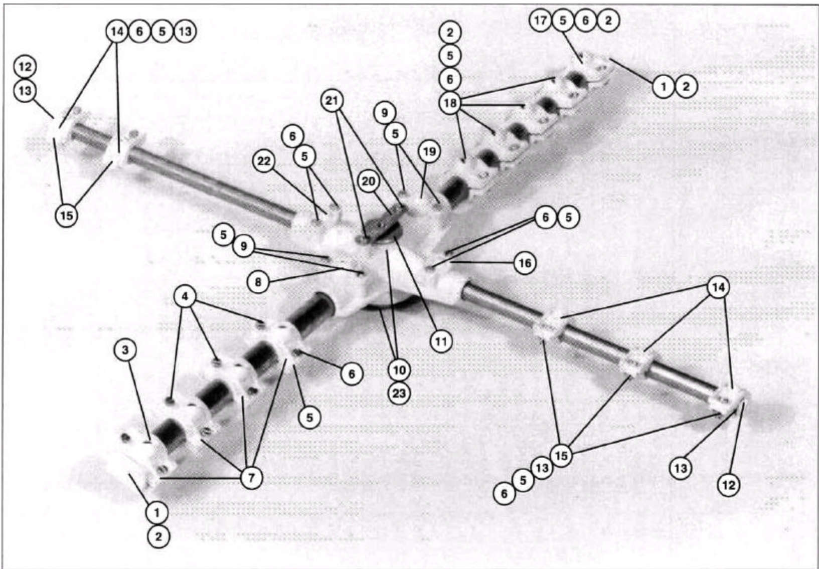
Fig. 26 - D-HB/D-HI/D-LF Wash/Rinse Spray Arms (For machines built prior to S/N 77854)
