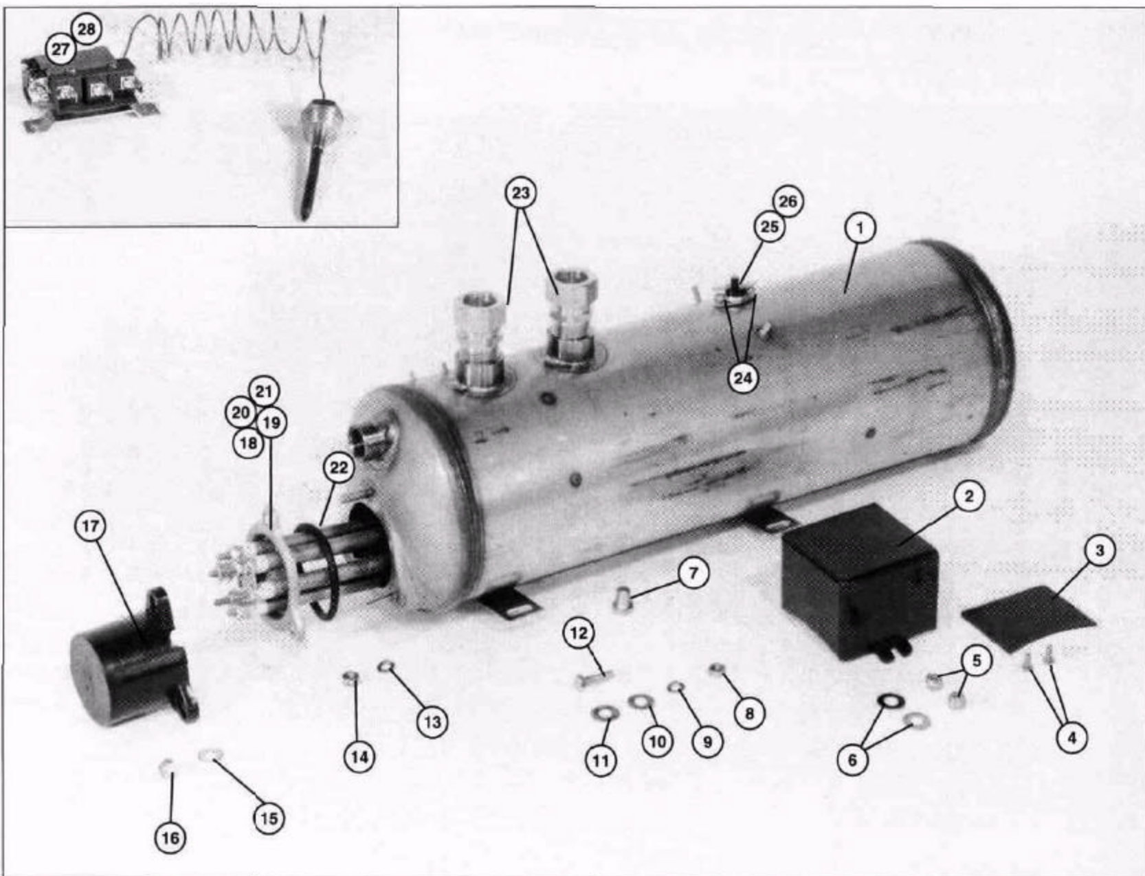
Fig. 31 - D-HB Electric Booster Assembly and Thermostat
