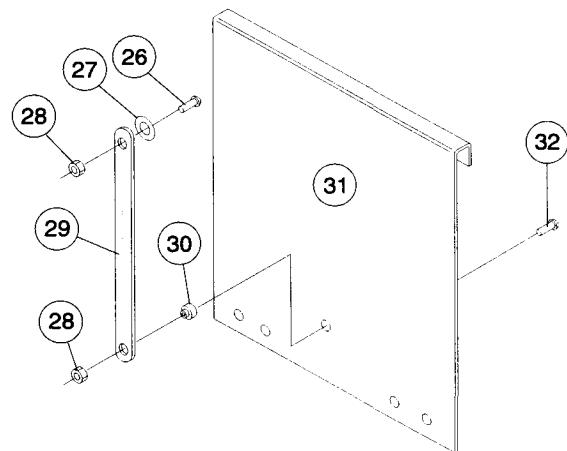
Fig. 22 - D-HB/D-H1/D-LF Door Linkage For machines beginning with S/N 13809 and above
