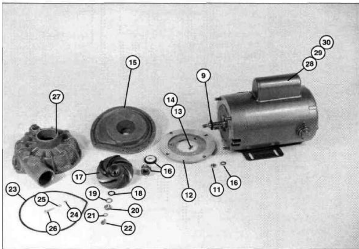
Fig. 30 - D-HB/D-H1/D-LF Pump Assembly
