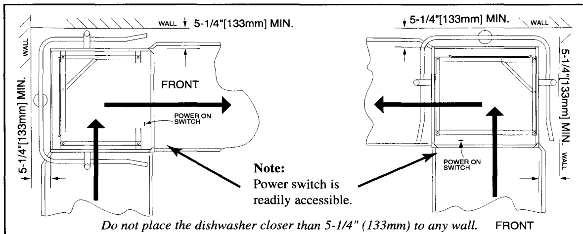
Figure 1 Placement for Corner Operation
