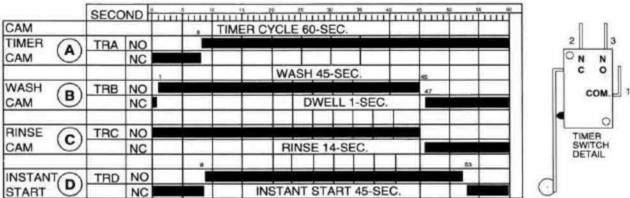
Figure 13 Cycle Timer Chart
