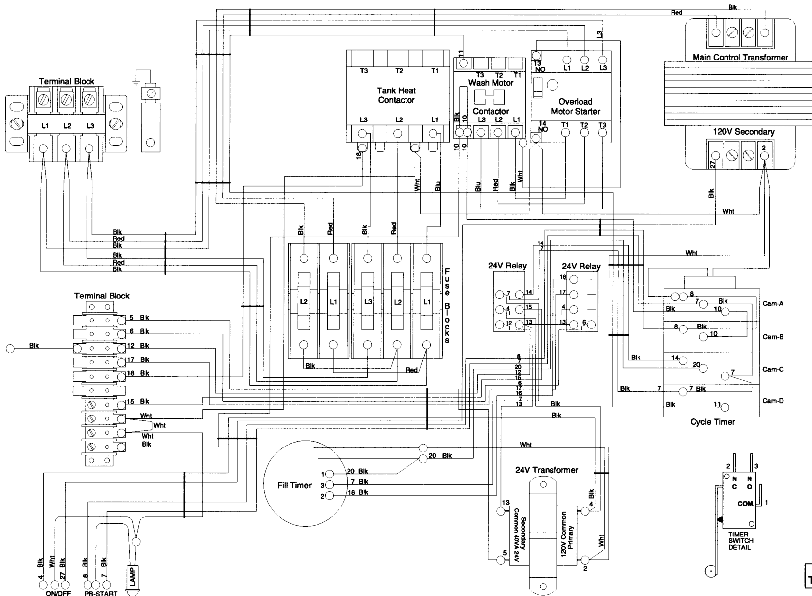
Fig. 41 – Wiring Diagram D-H1/D-LF, 3 Phase
