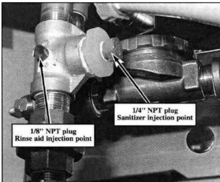
Figure 7 D-LF Rinse Aid/Sanitizer Injection Points
