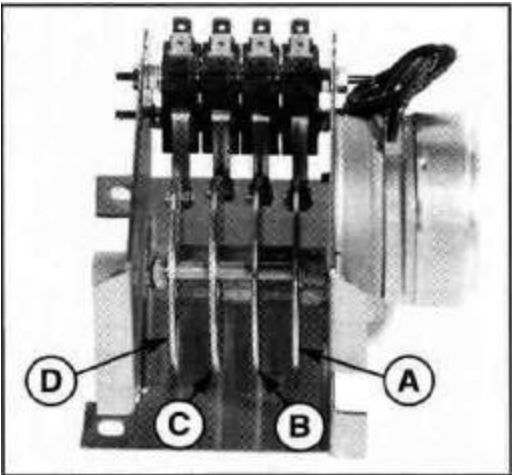
Figure 12 Cycle Timer
