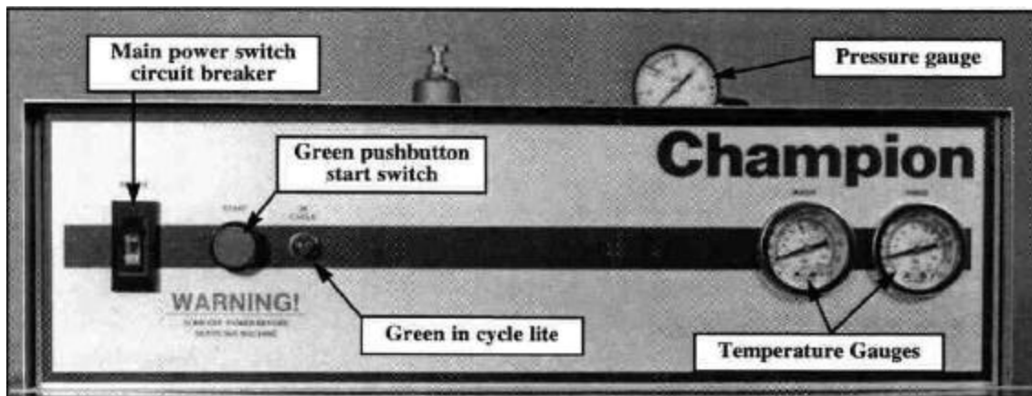
Figure 8 Operator Controls Top Mounted Control Cabinet
