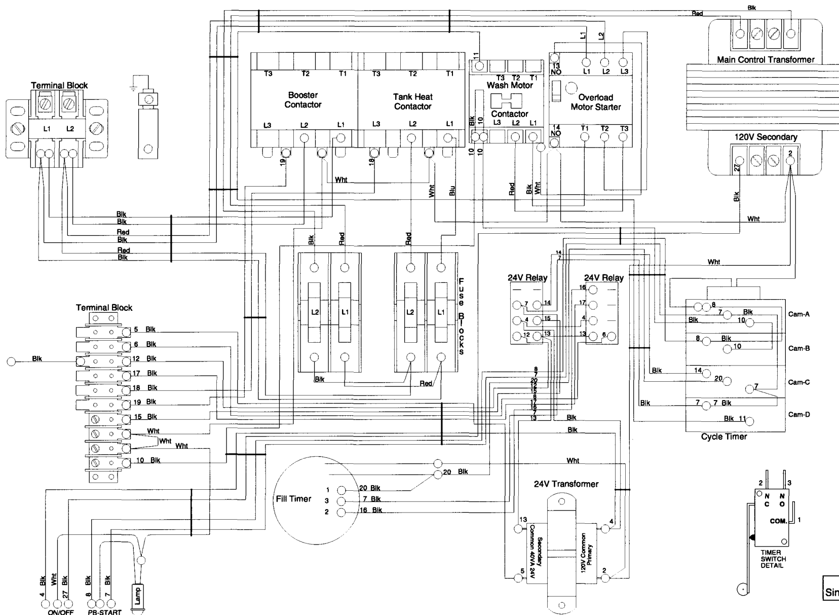
Fig. 40 - Wiring Diagram D-HB, 1 Phase
