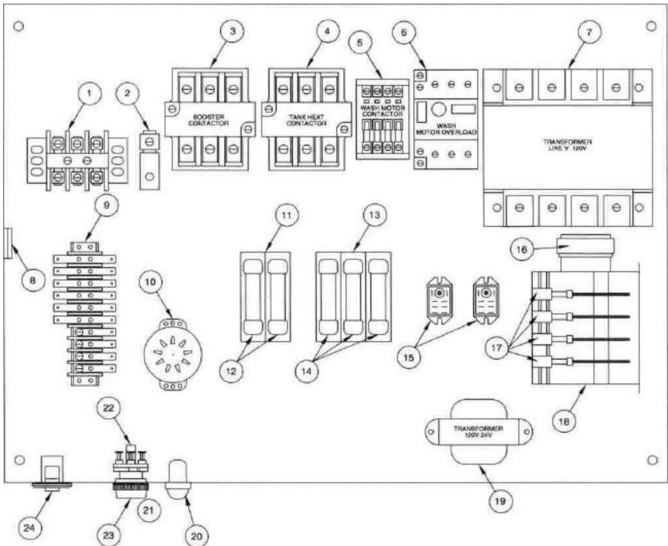
Fig. 32 - D-HB/D-H1/D-LF Control Cabinet
