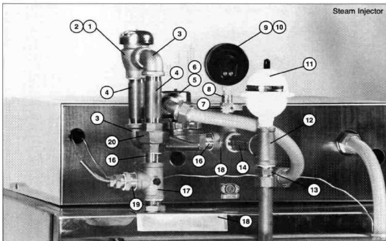
Fig. 34 - D-HB Steam Coil/Steam Injector Fill Piping
