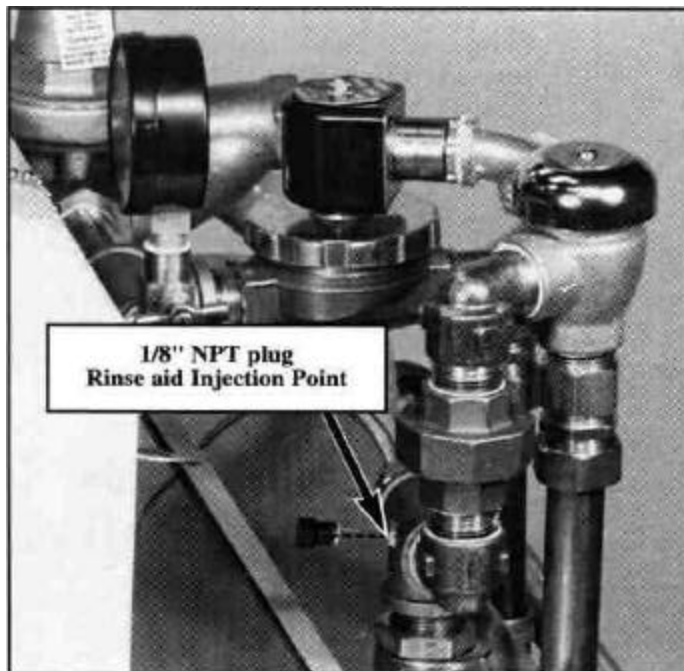
Figure 6 Rinse aid Insertion Point D-HB, D-H1 Only
