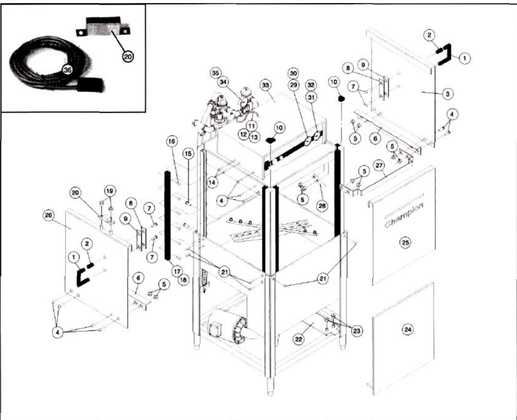
Figure 20 - D-HB/D-HI/D-LF Doors, Panels and Gauges
