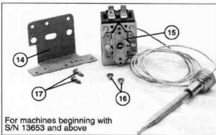
Fig. 27 - D-HB/D-H1/D-LF Tank Heater Element and Thermostat
