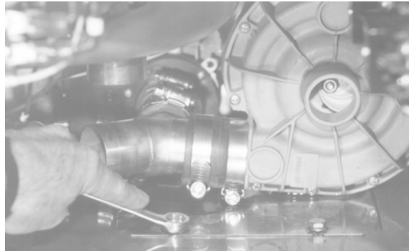
Remove hoses Remove (2) retaining bolts
