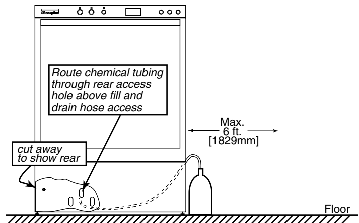
Figure 2.9.3 Chemical Bottle Placement
