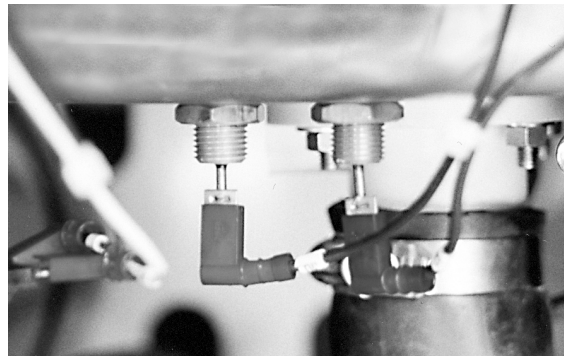
Remove heater leads and retaining nuts
