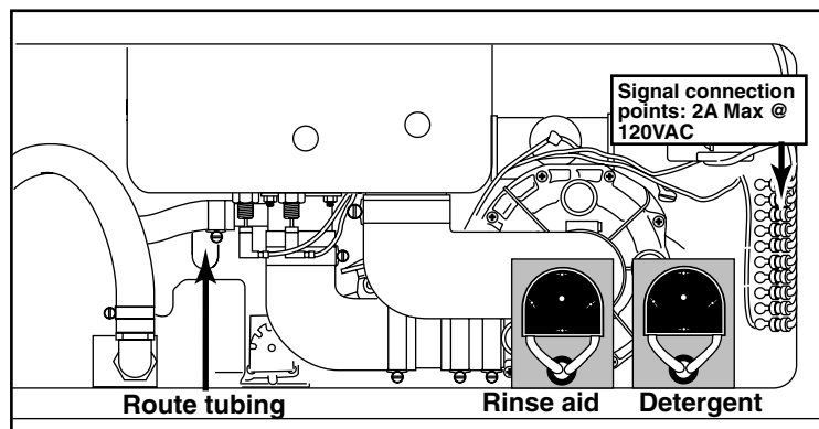
Figure 2.10.3 UH-100B, UH-100 Chemical Pumps
