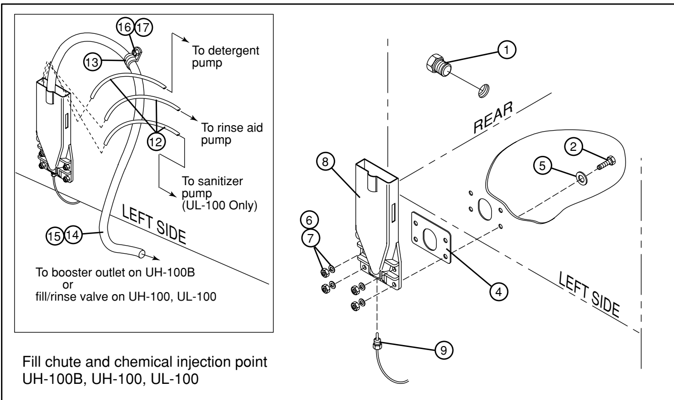
Figure 9.6- Chemical Injections Points, Water Level Probe Assembly (UH-200B, UH-200) and Fill Chute Assembly (UH-100B, UH-100, UL-100)
