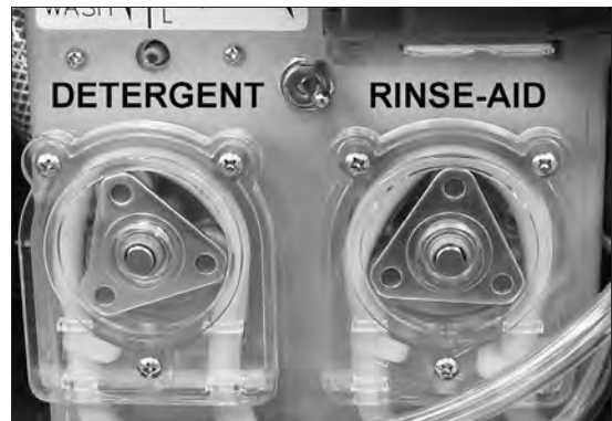
For Models UH100B and UH100, the dispensing pumps are located on the center bracket behind the lower-front access panel.
