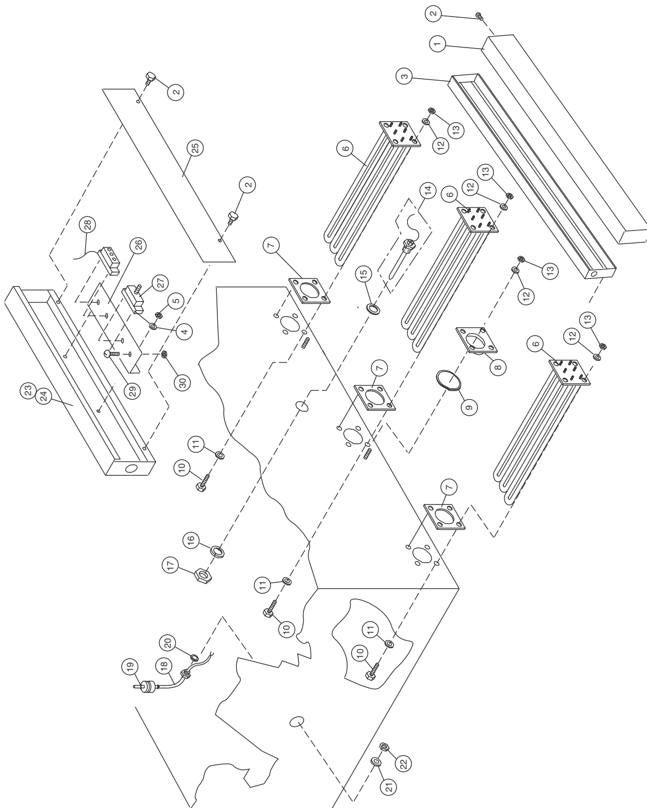
Figure 6.9a- Electric Tank Heat (For machines beginning with S/N J1050 and above)
