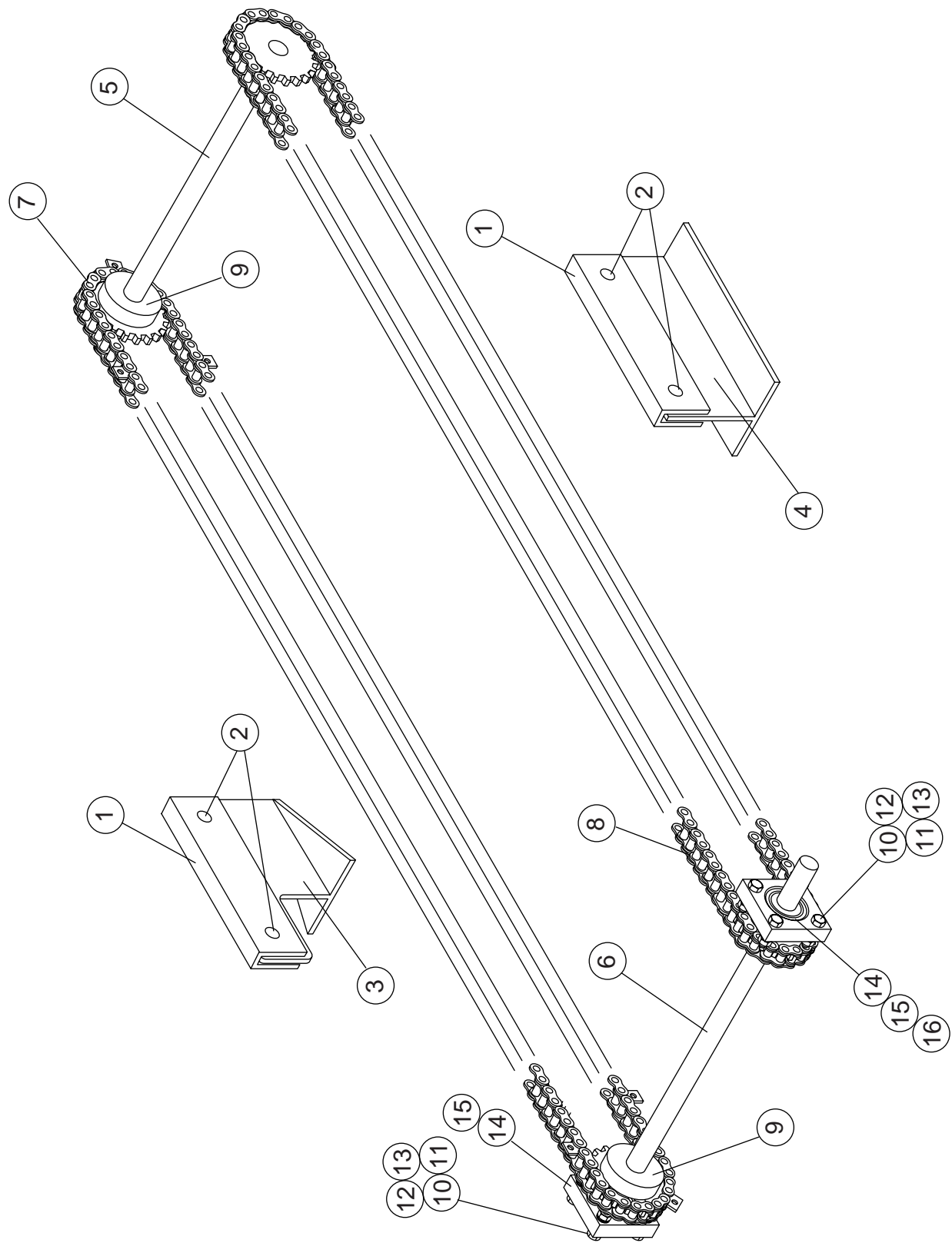
Figure 6.5 - Conveyor shafts, chains, bearings, and guides (For machines built prior to S/N J1050)
