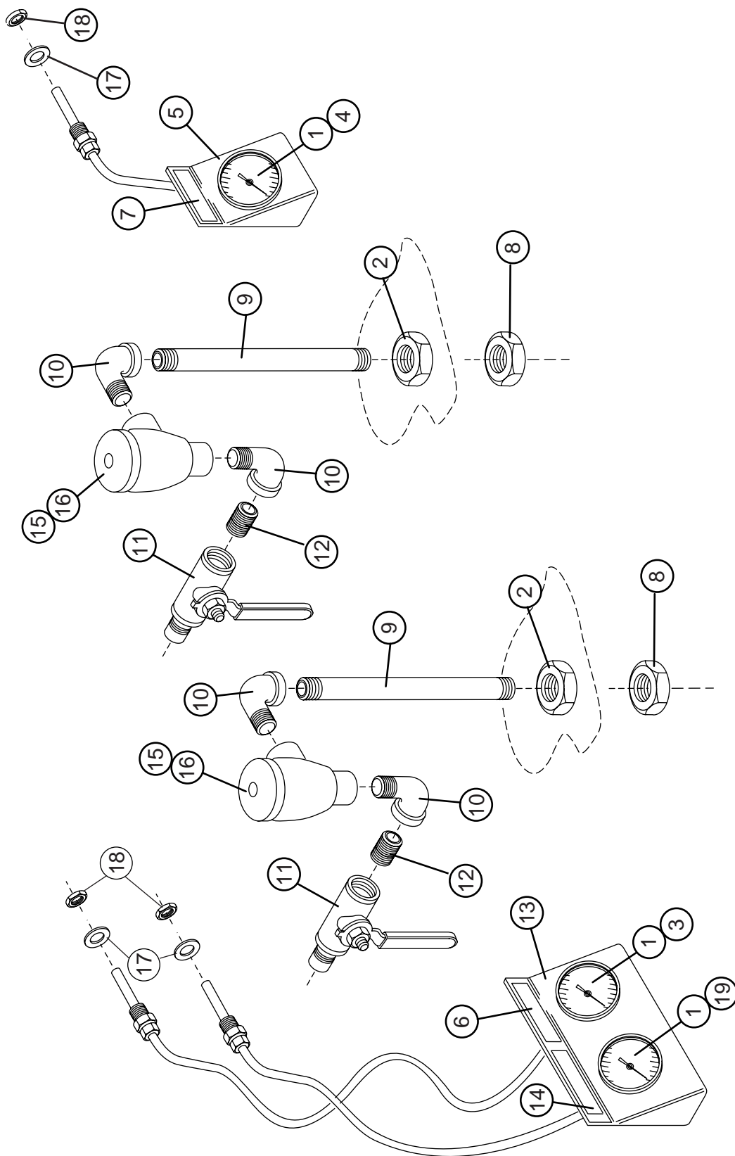
Figure 6.2 - Tank fill assembly and Temperature gauges (R-L machine shown)
