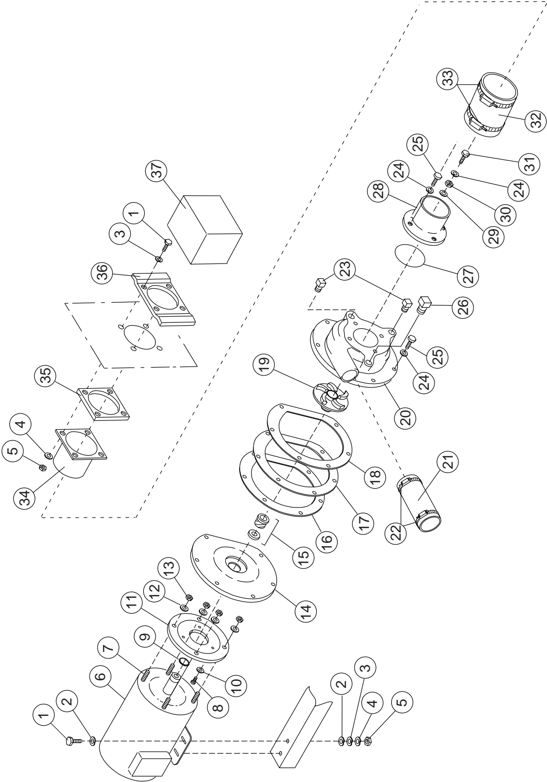
Figure 6.13 - Pump assembly
