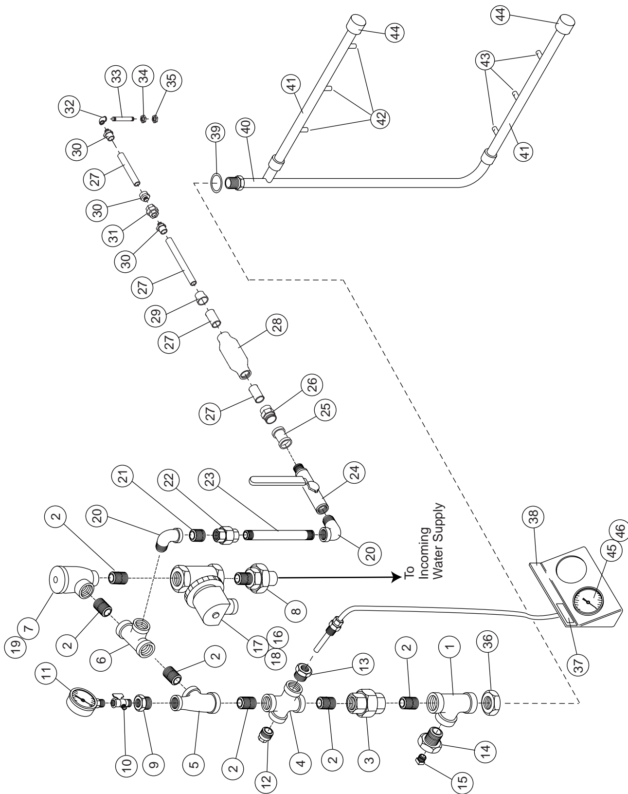
Figure 6.3 - Final rinse piping assembly (R-L machine shown)
