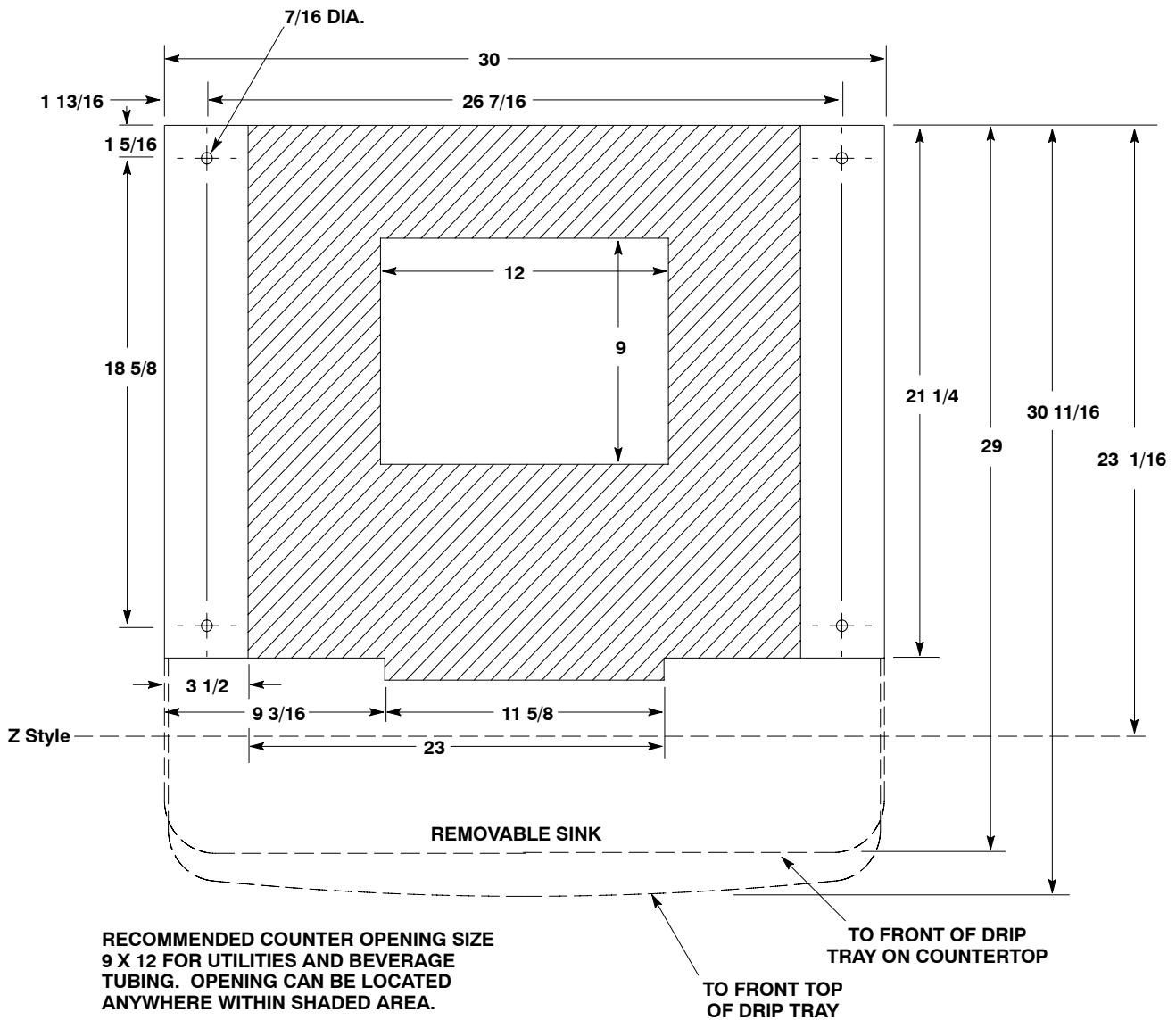
FIGURE 3. MOUNTING TEMPLATE
