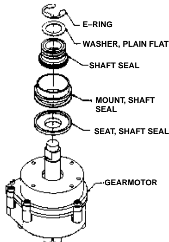
FIGURE 19. SHAFT SEAL 700 & 1000
