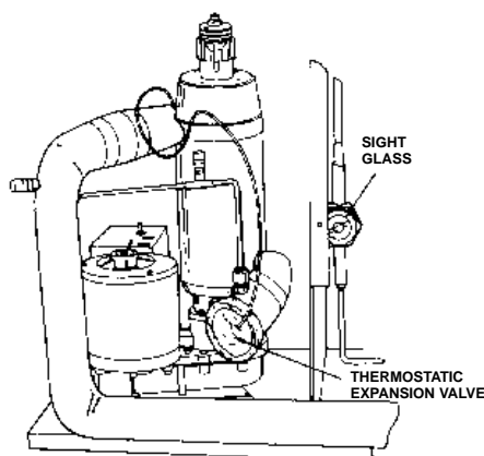
FIGURE 13. EXPANSION VALVE
