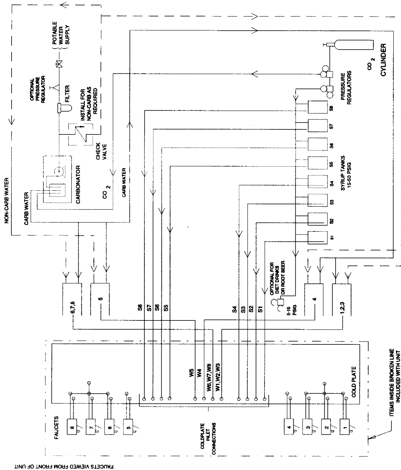
FIGURE 2. FLOW DIAGRAM
