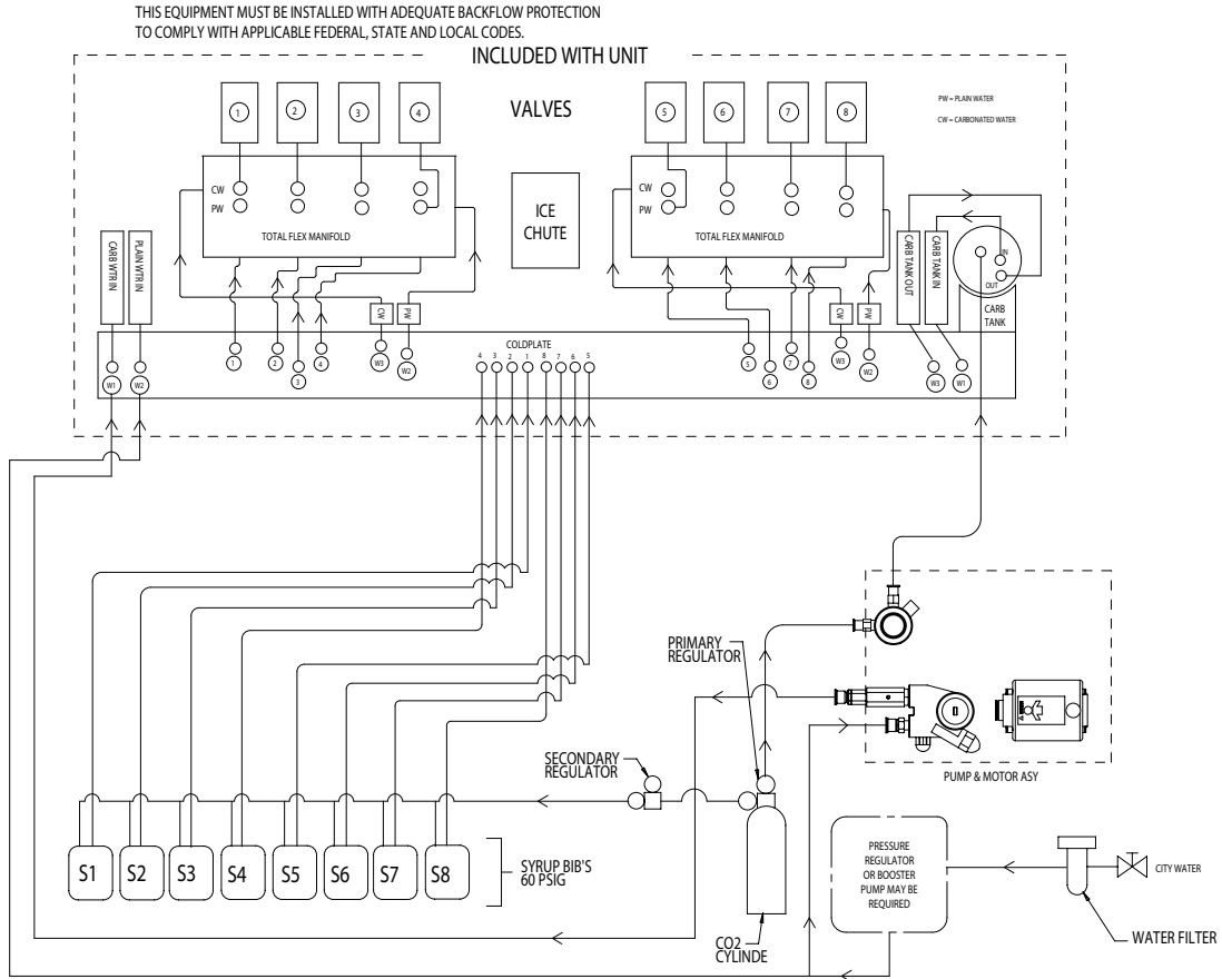
Figure 4. Flow Diagram - Eight Flavor Unit
