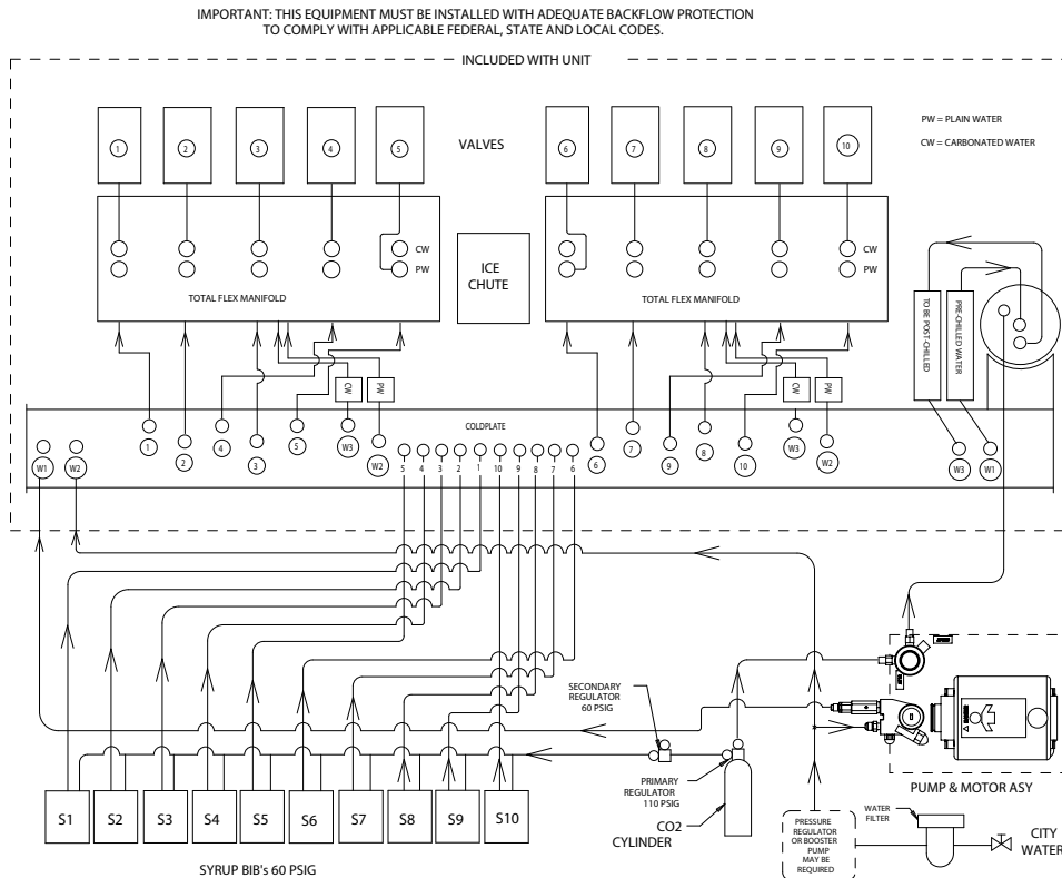
Figure 5. Flow Diagram - Ten Flavor Unit
