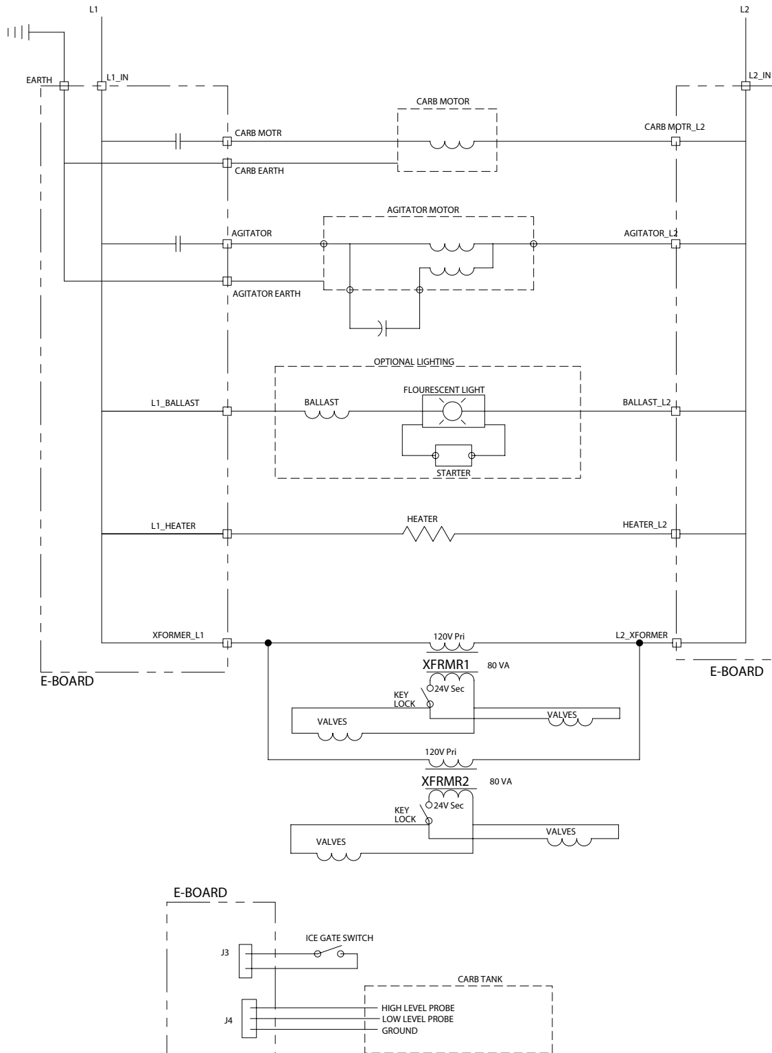
Figure 8. Wiring Schematic
