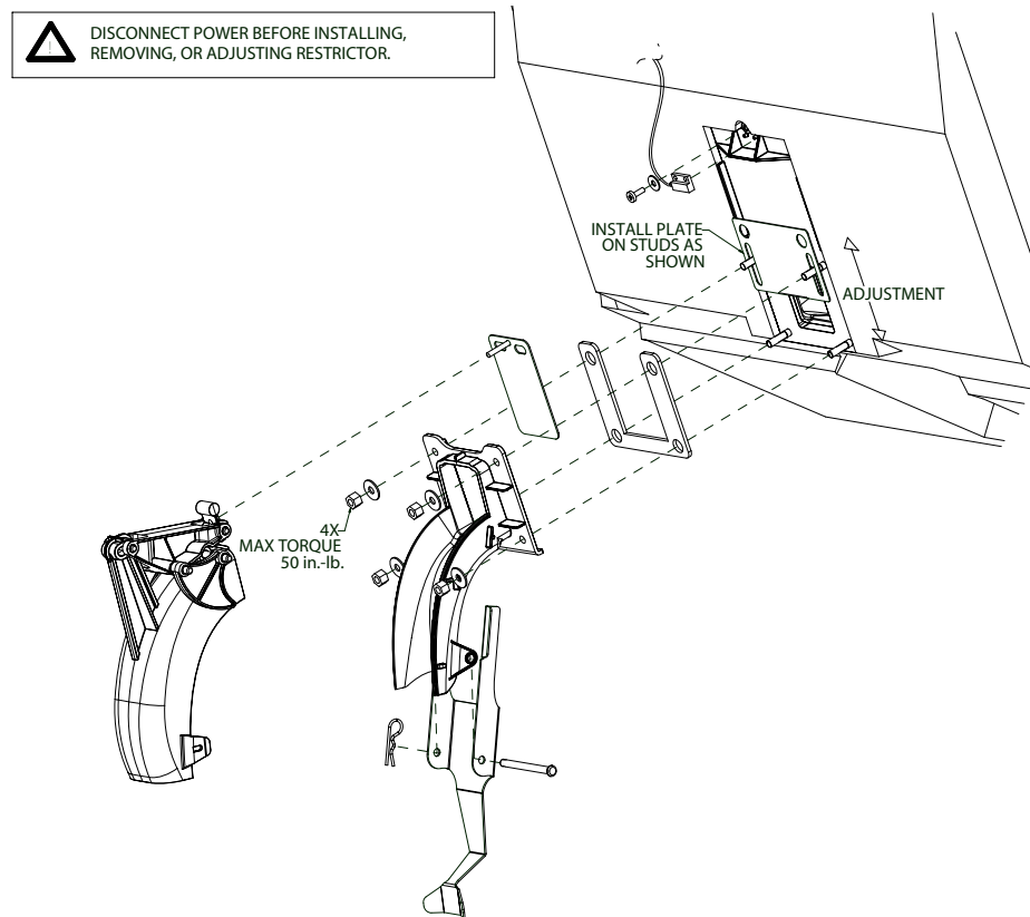
Figure 1. Gate Restrictor Plate
