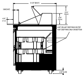
D4460N-18M Right Side View
