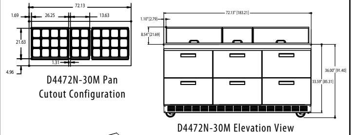
D4472N-30M Elevation View
