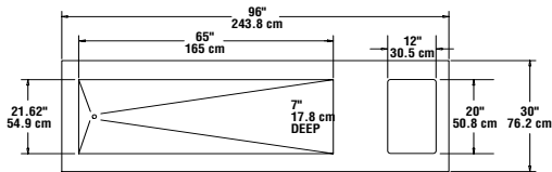
PLAN VIEW KHC-96-NU
