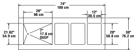
PLAN VIEW KH3C-74-NU
