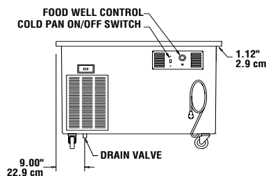
TYPICAL ELEVATION VIEW ALL MODELS
