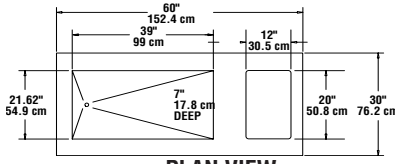
PLAN VIEW KHC-74-NU
