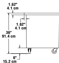
RIGHT END VIEW ALL MODELS
