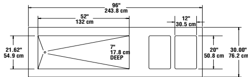
PLAN VIEW KH2C-96-NU
