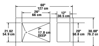
PLAN VIEW KHC-50-NU
