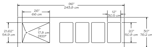
PLAN VIEW KH4C-96-NU
