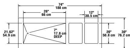
PLAN VIEW KH2C-74-NU
