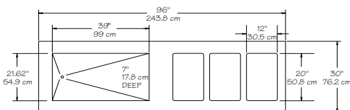
PLAN VIEW KH3C-96-NU
