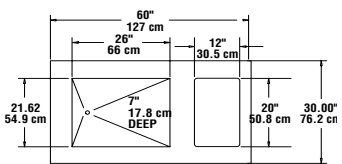
PLAN VIEW KHC-60-NU
