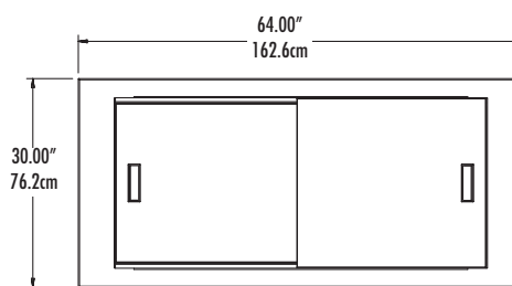
Plan View SPH-64E
