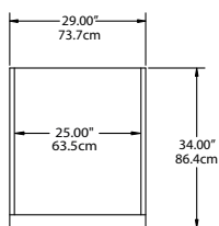
PLAN VIEW SSF1-S, SAF1-S, SMF1-S SSF1-SH, SAF1-SH, SMF1-SH
