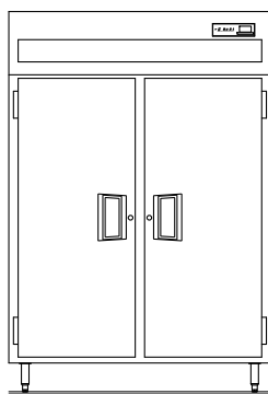
ELEVATION VIEW SSF2-S, SAF2-S, SMF2-S
