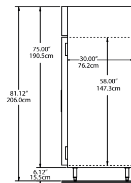
END VIEW 1 & 2 SECTION MODELS
