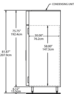
END VIEW 3 SECTION MODELS
