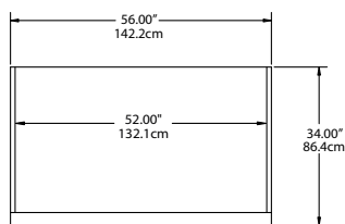
PLAN VIEW SSF2-S, SAF2-S, SMF2-S SSF2-SH, SAF2-SH, SMF2-SH
