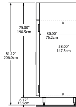
END VIEW 1 SECTION UNITS
