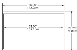
PLAN VIEW SSRPT25-S, SARPT25-S, SMRPT25-S SSRPT25-SH, SARPT25-SH, SMRPT25-SH
