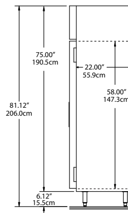
End View All Models
