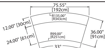
DCRUI-TT32 Plan View
