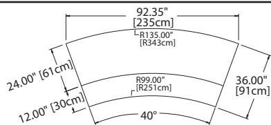
DCRUI-TT40 Plan View
