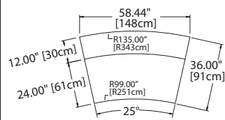
DCRUI-TT25 Plan View
