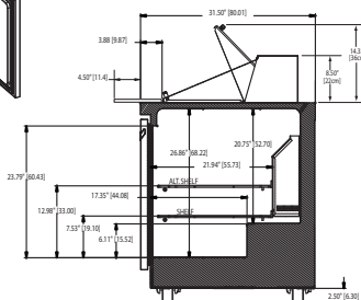
4460N-18M Right Side View
