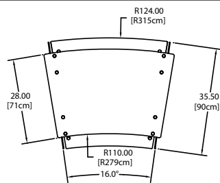
DCFSRKD-2 Plan View
