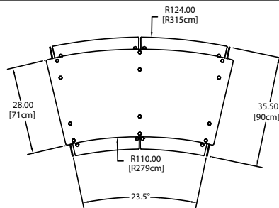
DCFSRKD-3 Plan View
