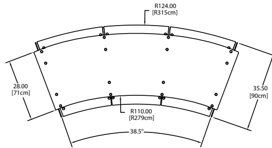
DCFSRKD-5 Plan View
