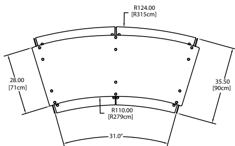
DCFSRKD-4 Plan View
