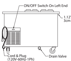
Elevation View KCM-50
