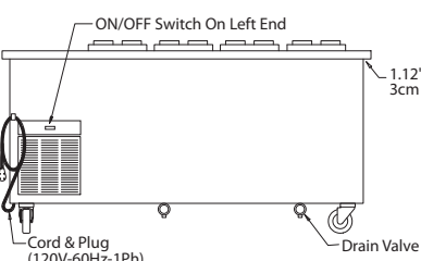
Elevation View KCM-74
