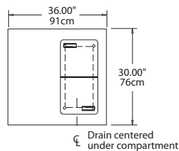
Plan View KCM-36
