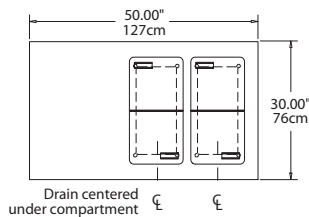
Plan View KCM-50
