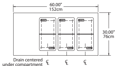
Plan View KCM-60
