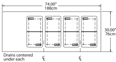
Plan View KCM-74
