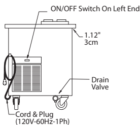
Elevation View KCM-36
