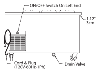
Elevation View KCM-60
