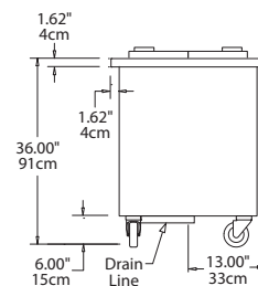
End View All Models
