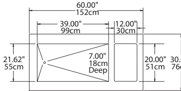
Plan View SHC-60-NU
