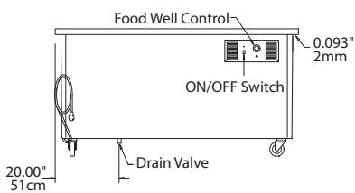
Typical Elevation View All Models
