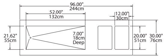
Plan View SH2C-96-NU
