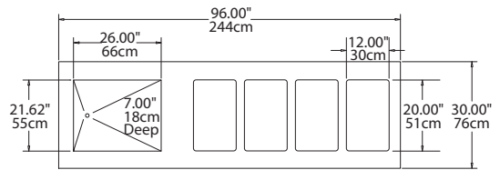
Plan View SH42C-96-NU
