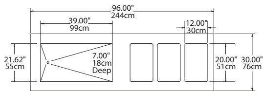
Plan View SH3C-96-NU
