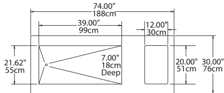
Plan View SHC-74-NU
