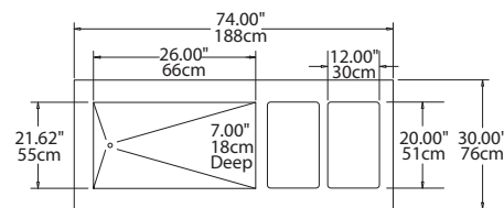
Plan View SH2C-74-NU
