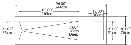
Plan View SHC-96-NU
