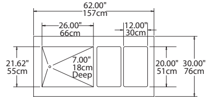
Plan View SH2C-62-NU
