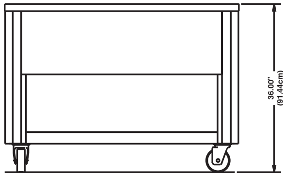
ELEVATION VIEW
