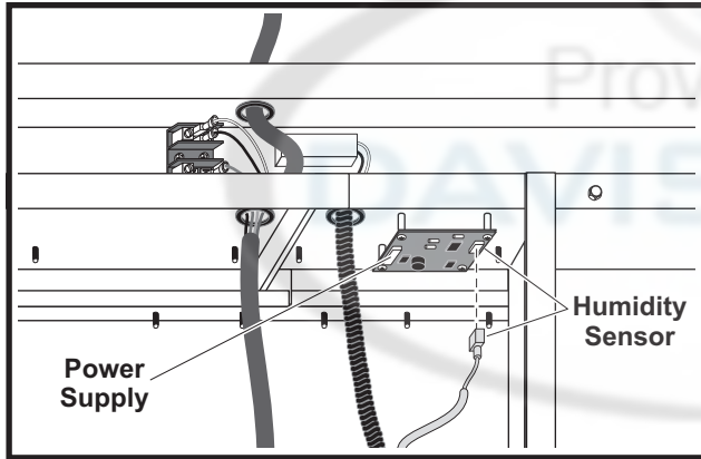
Figure 27: Location of the Humidity PC Board
