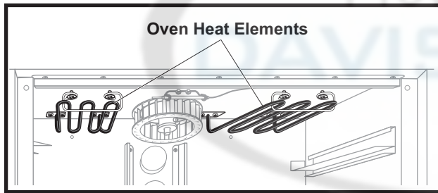
Figure 30: View of Oven with Oven Ceiling Panel Removed
