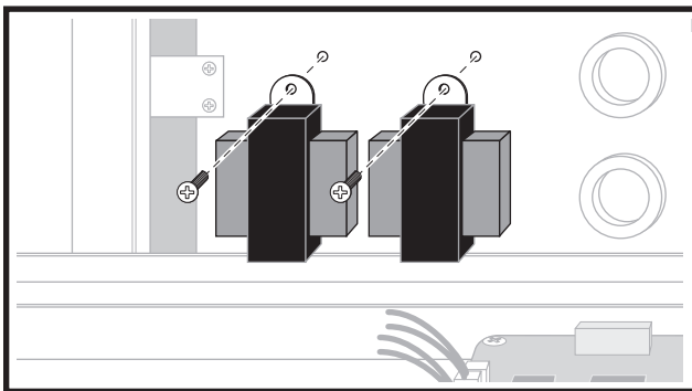
Figure 15: Proofer &amp; Oven Light Transformers
