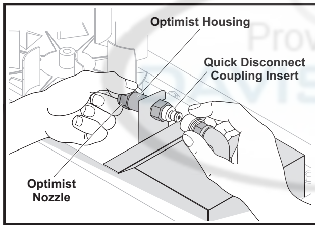
Figure 28: Optimist Nozzle Quick Disconnect
