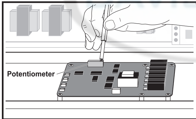
Figure 13: Brightness Adjustment Potentiometer
