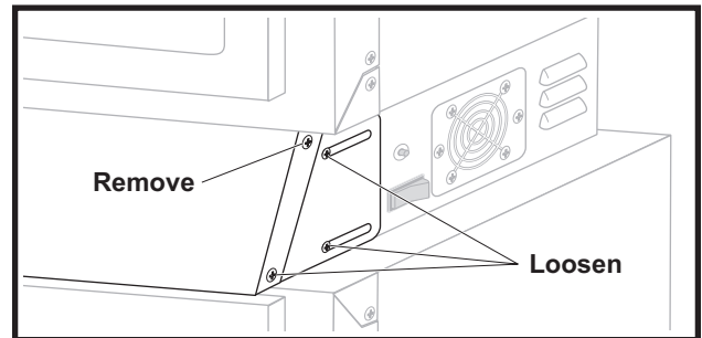
Figure 6: Electrical Component Access Panel Screw Locations
