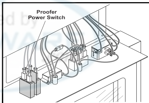
Figure 19. Location of Proofer Power Switch
