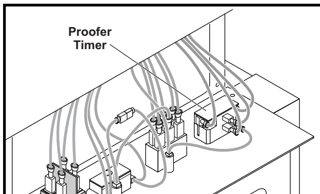
Figure 24. Proofer Heat Element Connections – Left Side Rear
