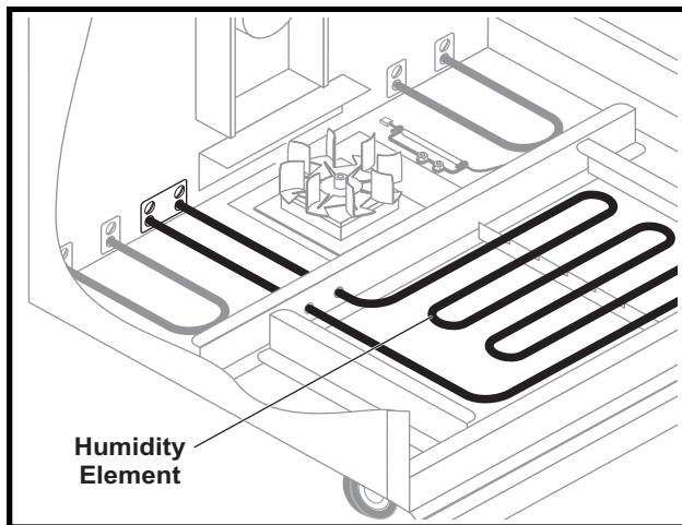
Figure 28. Location of Proofer Humidity Element
