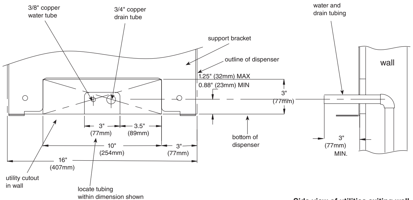
Side view of utilities exiting wall
