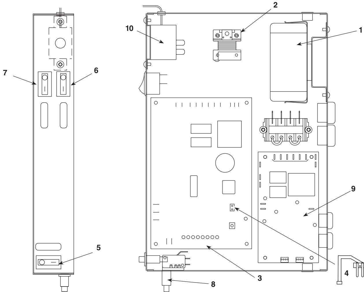
Side view
