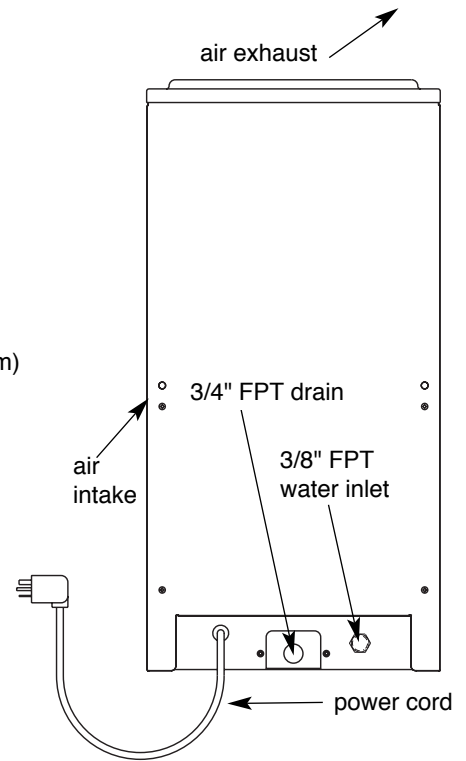
Dispenser rear view
