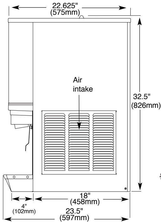
Dispenser side view
