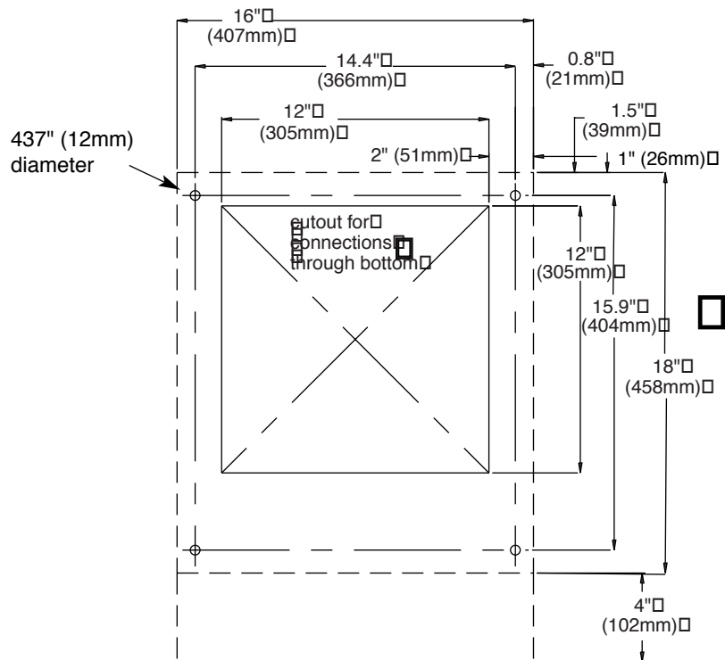
Fig. 1 – Counter information
