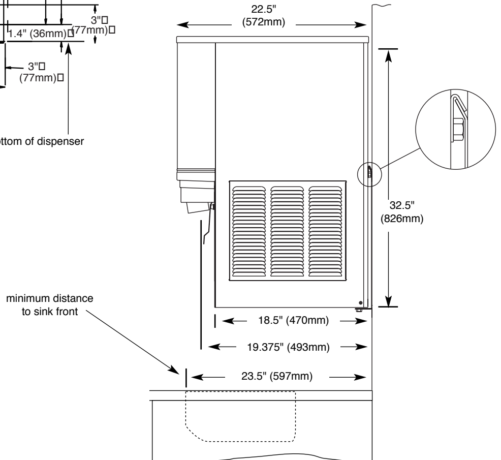
Fig. 7 – Wall mount side view
