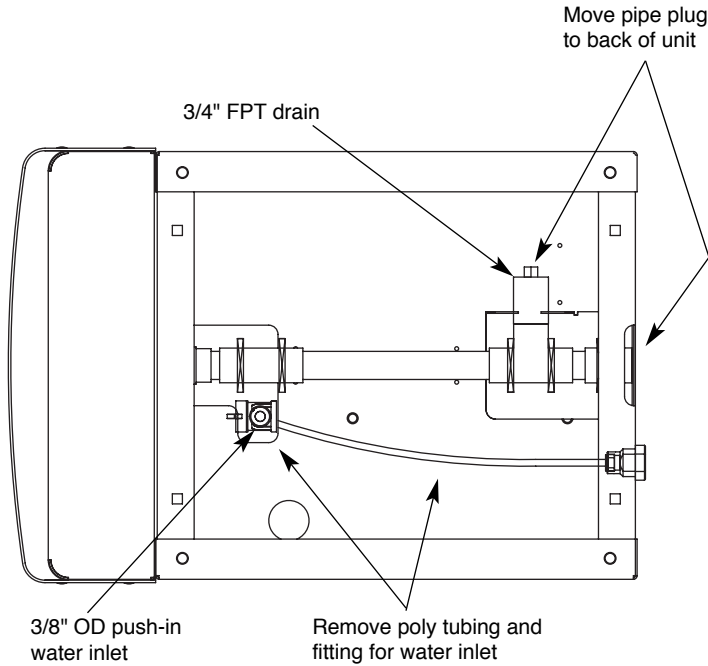
Fig. 2 – Bottom exiting utilities (countertop units)
