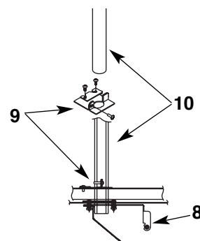
Ice tube bracket – side view – all top mounted units
