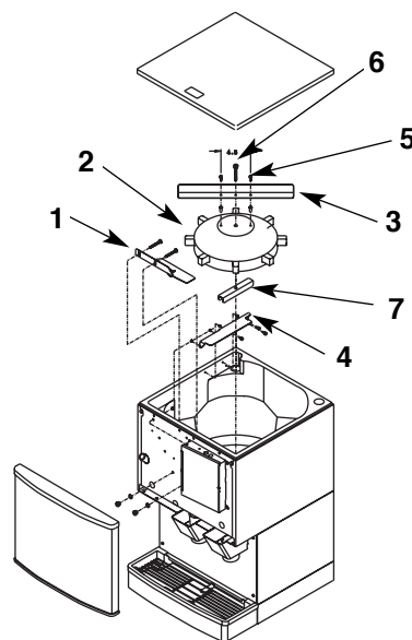
Top view – freestanding and Satellite-fill units
