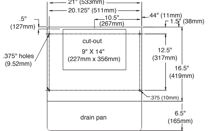
Fig. 2 – Counter cut-out, all models
