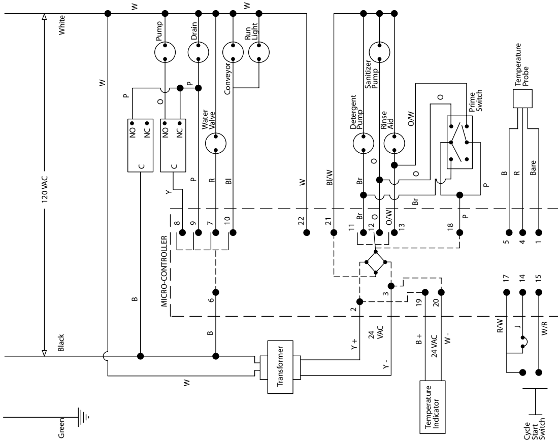
GT-18 Wiring Diagram
