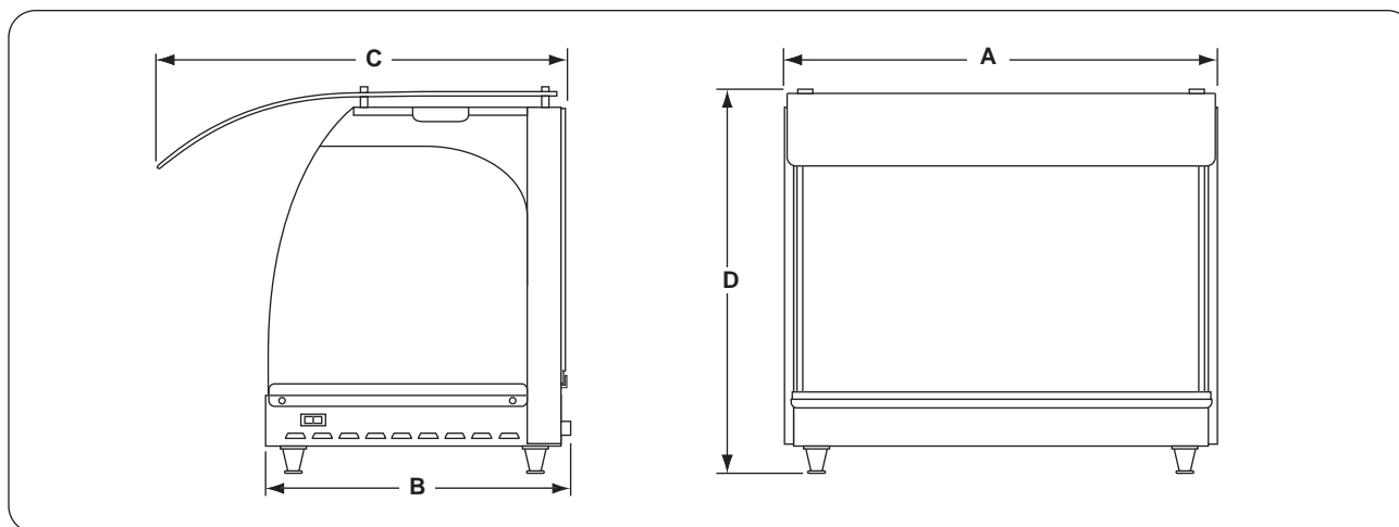
Figure 4. Dimensions Glo-Ray Model GRCMW-1
