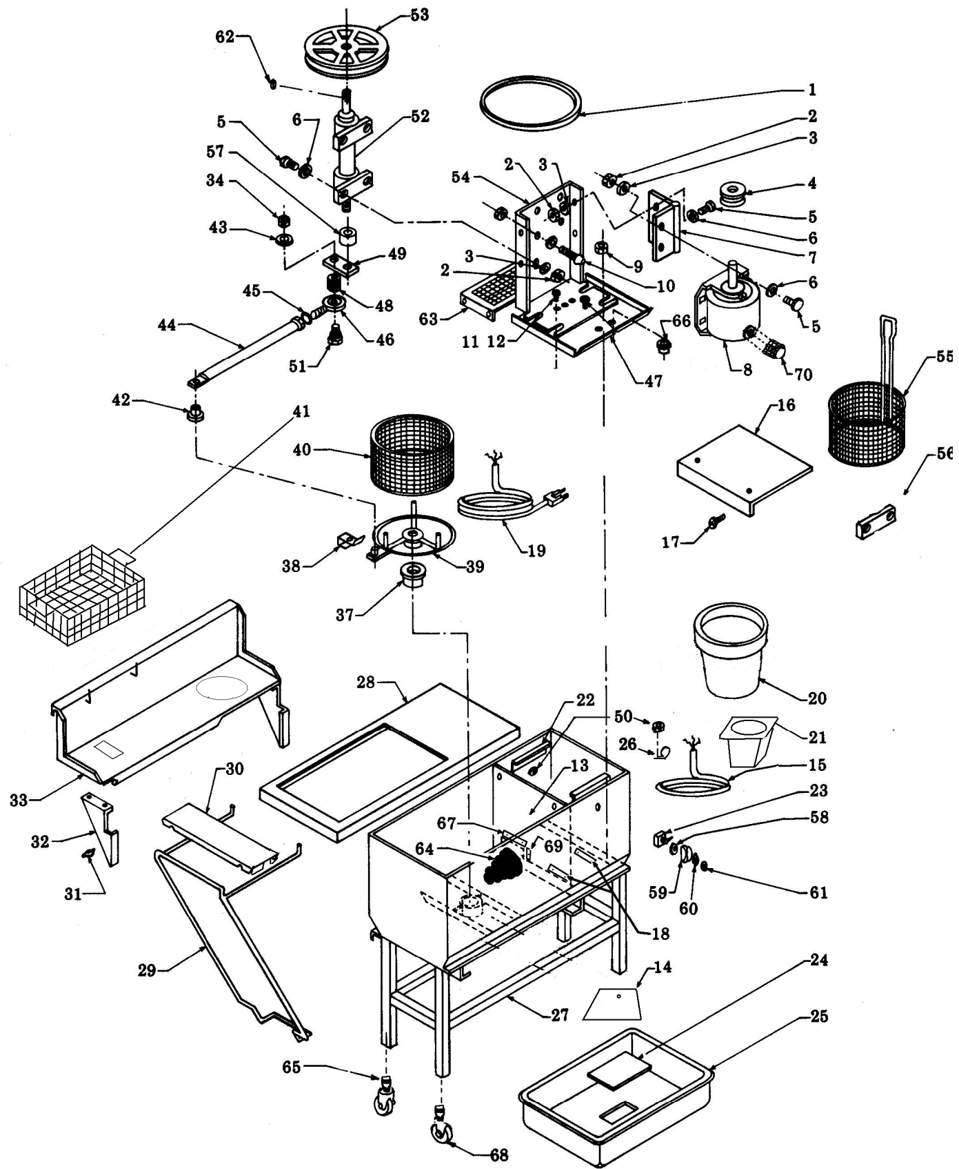
EXPLODED VIEW OF HB-11 HAND BREADER/SIFTER
