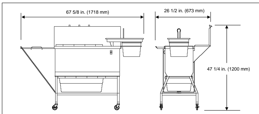
Model HB-121 hand breader/sifter configured for right to left work flow. (Sheet pan sold separately.)
