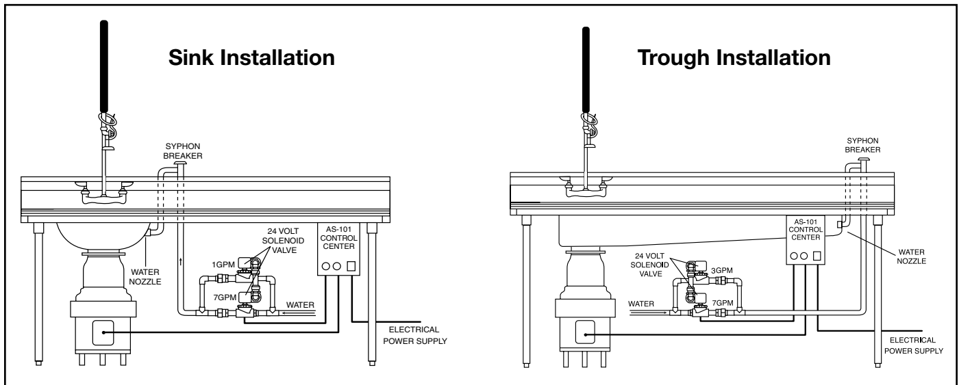
Figure 2. Typical Installation Diagram
