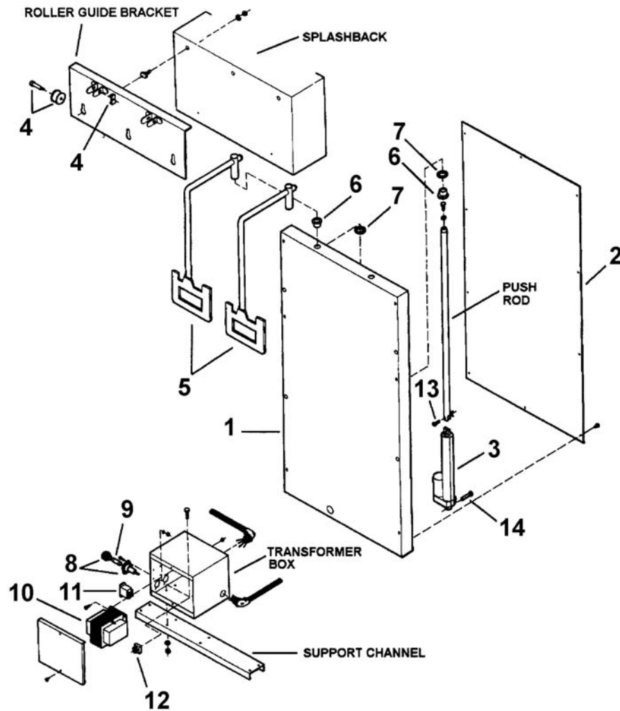
Figure 6-5 18" - 24" Basket-Lift Housing, Roller Guide and Transformer Box
