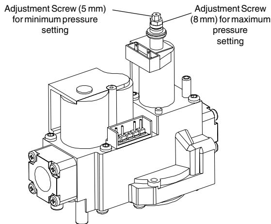
Figure 2-18. Gas Valve
