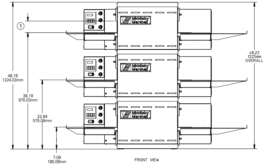
Figure 2-7. MODEL 520 TRIPLE OVEN DIMENSIONS
