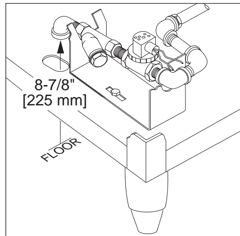
DH1T, DH1TC 3/4" NPT Hot Water Connection
