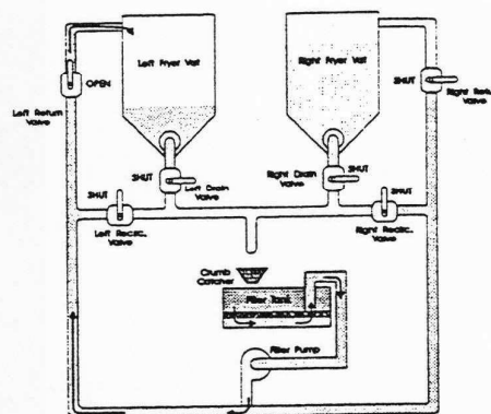
RETURN MODE
