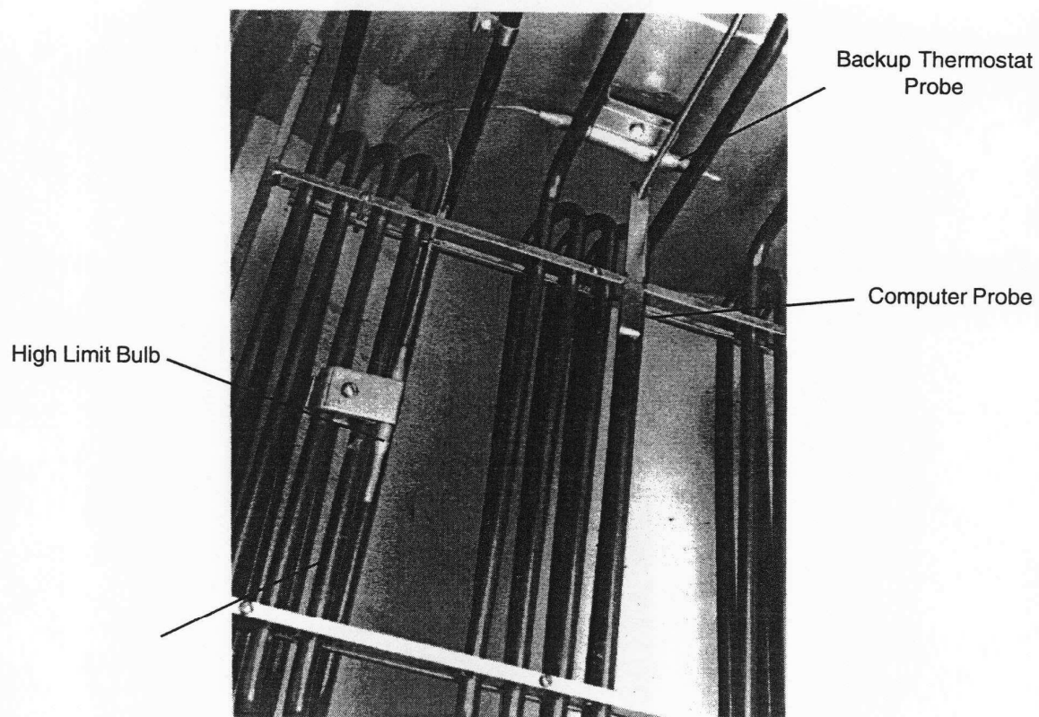
Heating Elements
