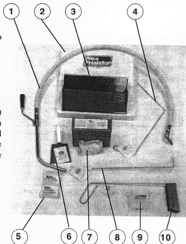
Figure 1-1 Filter Tools and Accessories
