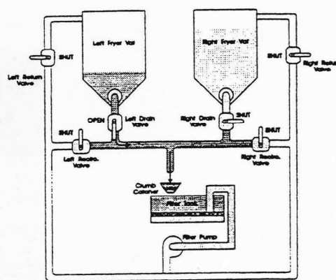
DRAIN MODE
