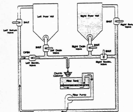
CIRCULATE MODE
