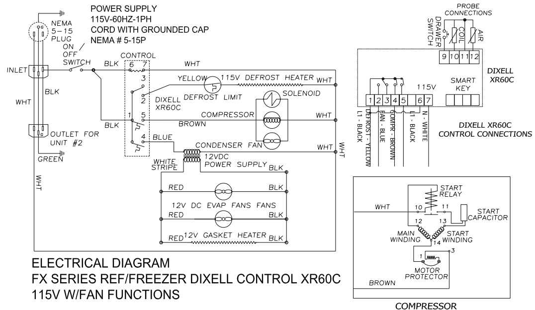
BOTTOM FX-1(2N1) ELECTRICAL DIAGRAM WITH DIXEL XR60C CONTROL WITH RED DISPLAY
