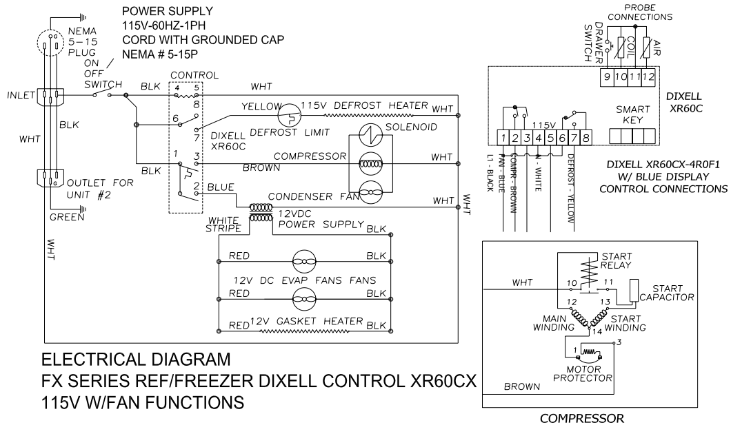
TOP FX-1(2N1) ELECTRICAL DIAGRAM WITH DIXEL XR60CX CONTROL WITH BLUE DISPLAY
