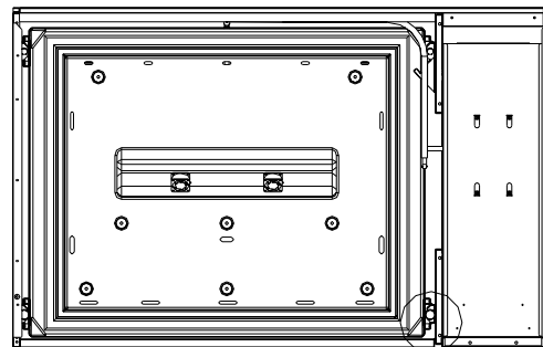
BOTTOM VIEW OF EVAPORATOR LID ASSEMBLY (CABINET BOTTOM AND DRAWER ASSEMBLY REMOVED FOR CLARITY)
