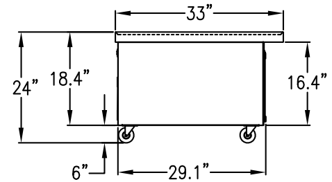
SIDE VIEWS
