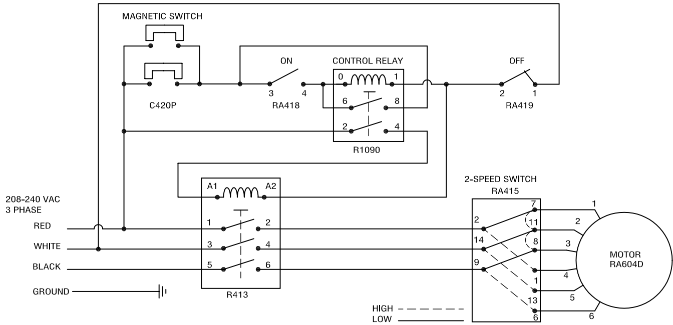
Models R4N & R6N Wiring Diagram USA Machines with Metal Base 220V, 3 Ph, 850/1725 RPM, .5/1.0 HP, 3.2/3.0 Amps
