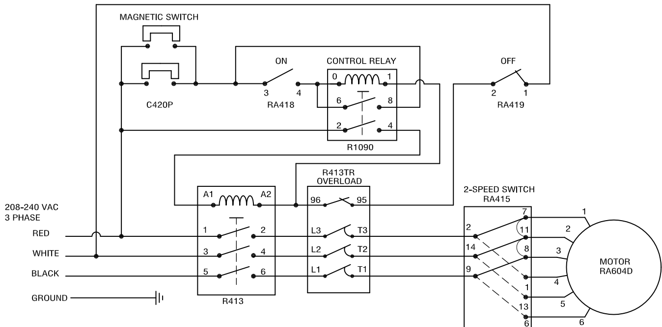
Models R4N & R6N Wiring Diagram Canadian with Metal Base 220V, 3 Ph, 850/1725 RPM, .5/1.0 HP, 3.2/3.0 Amps
