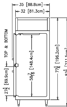
Section - HT132NUT
